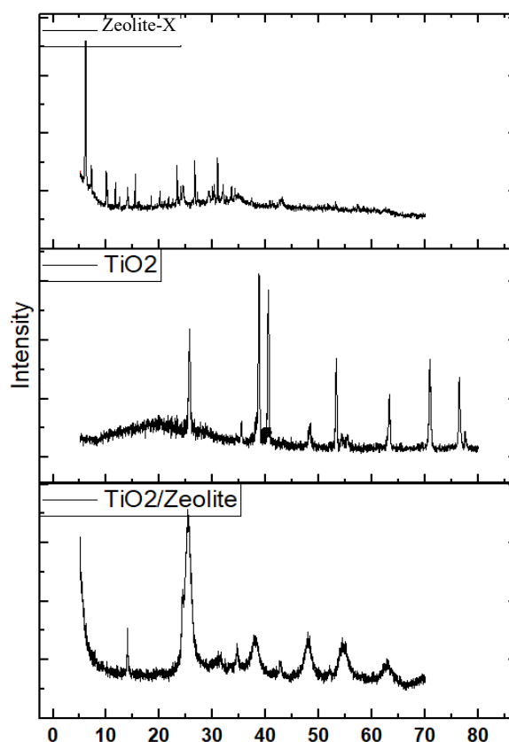
Figure 5. X-ray diffraction patterns of zeolite, \text{TiO}_2 , and the nanocomposite \text{TiO}_2/\text{zeolite}
