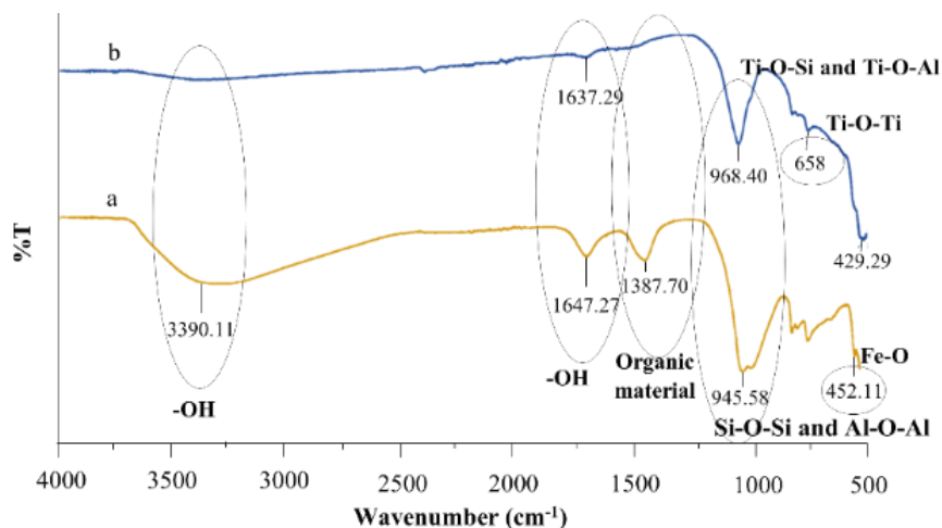
Figure 3. FTIR spectrum (a) Zeolite synthesized from coal fly ash waste; (b) TiO 2 /zeolite nanocomposite
