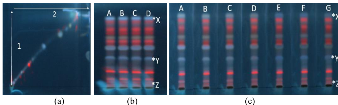
Figure 3. (a) TLC chromatogram of analyte stability test during chromatography (1) First solvent development process, (2) Second development process. (b) TLC chromatogram of the analyte stability test on the plate and in solution in (A) lane 1, (B) lane 2, (C) lane 3, and (D) lane 4. (c) TLC chromatogram of analyte stability test visualization results on (A) 0 minutes, (B) 2 minutes, (C) 5 minutes, (D) 10 minutes, (E) 20 minutes, (F) 30 minutes, and (G) 60 minutes. For images (b) and (c), observations were made on three bands in the J. gendarussa leaf extract, which represent the top (X), middle (Y), and bottom (Z) areas.
