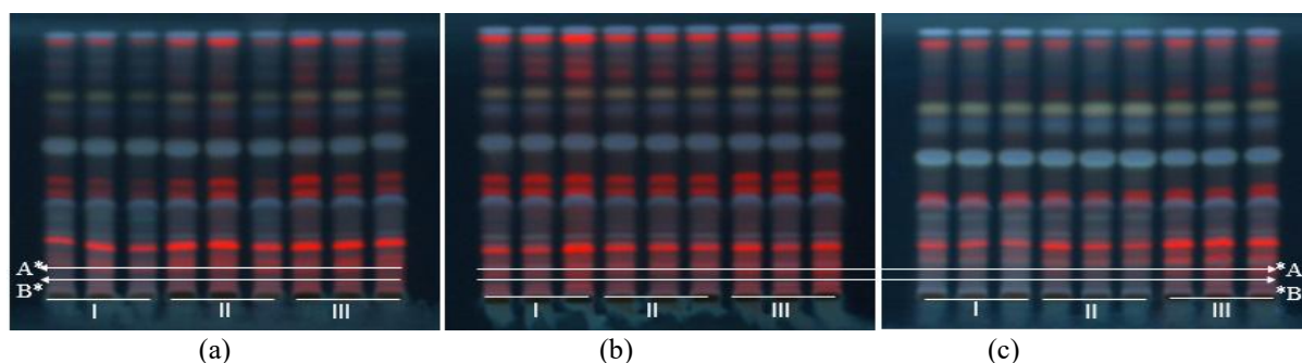
Figure 8. (a) Chromatogram of TLC fingerprint analysis on J. gendarussa leaf extract from Bogor, (b) Cianjur, and (c) Sukabumi areas from three genotypes of green and white leaves (I), green (II), and black stems (III).
