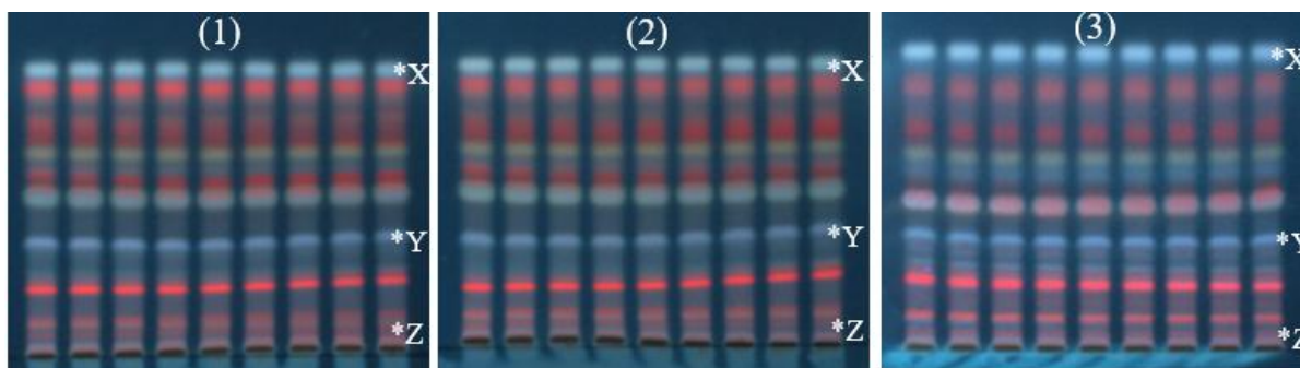
Figure 5. TLC chromatogram of precision determination on the same day (1) first plate, (2) second plate and (3) third plate
