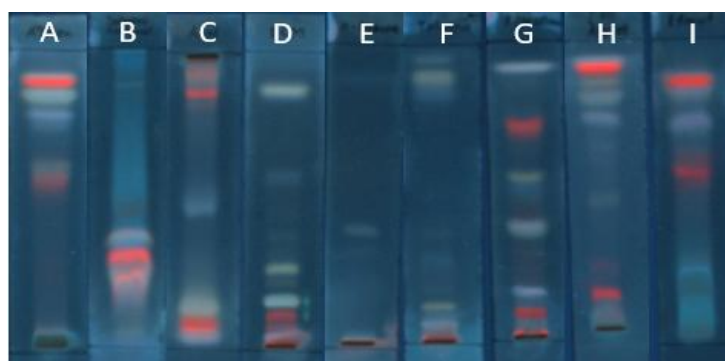
Figure 1. TLC chromatogram from J. gendarussa leaves extract using single eluent (A) acetone, (B) methanol, (C) acetonitrile, (D) DCM, (E) n-hexane, (F) toluene, (G) chloroform, (H) ethyl acetate, (I) ethanol.
