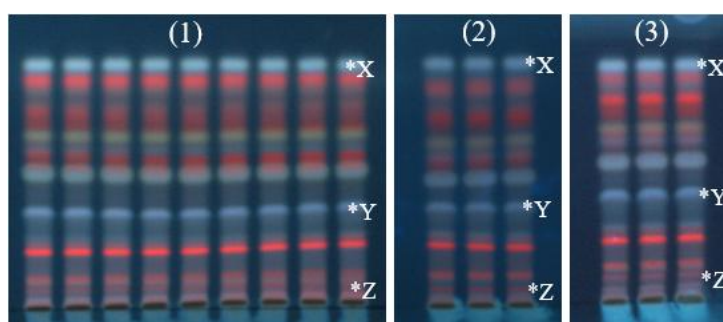
Figure 6. TLC chromatogram for determining precision on different days (1) first day, (2) second day, and (3) third day
