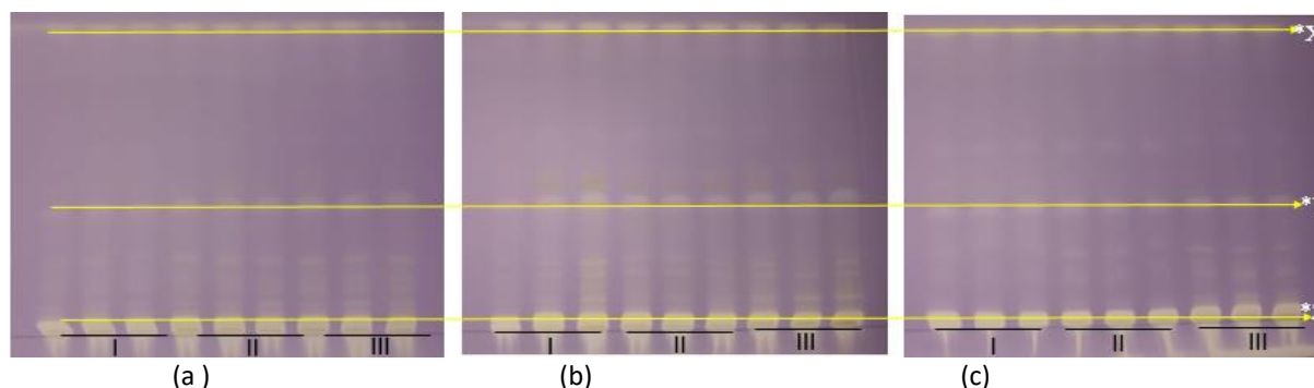
Figure 12. (a) TLC bioautography of antioxidants on leaf extracts from the Bogor, (b) Cianjur, and (c) Sukabumi areas from three genotypes of green and white leaves (I), green stems (II), and black (III)
