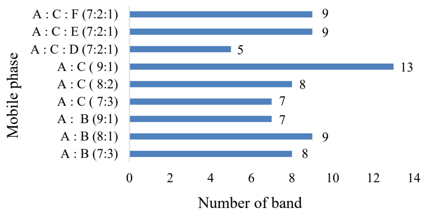
Figure 2. Results of mixed optimization of 2 and 3 mobile phases, such as chloroform (A), acetonitrile (B), ethanol (C), ethyl acetate (D), toluene (E), DCM (F) for TLC analysis of J. gendarussa leave extract based on the number of bands.
