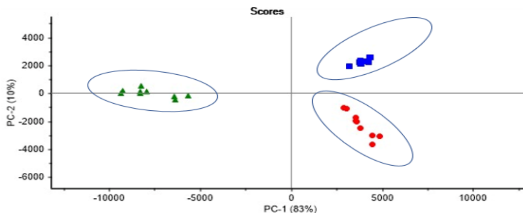
Figure 9. PCA score plot of J. gendarussa leaf extract with three types of genotypes from ■ the Bogor, ● Cianjur, and ▲ Sukabumi areas.
