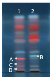
Figure 4. TLC chromatogram of specificity test on the extract of J. gendarussa leaves (lane 1) and R. simplex leaves (lane 2). Detection at a wavelength of 366 nm after adding sulfuric acid as a derivatization reagent.
