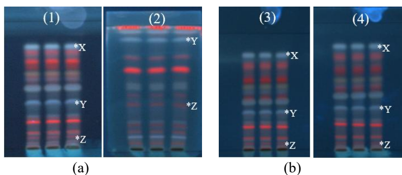
Figure 7. (a) TLC Chromatogram robustness test based on chamber type (1) twin-trough chamber, (2) flat bottom chamber and (b) Chromatogram of TLC robustness test based development distance (3) development distance of 7 cm, (4) development distance of 8 cm, in 3 bands on J. gendarussa leave extract representing the upper (X), middle (Y), and lower (Z) regions after derivatization in 366 nm UV light detection.
