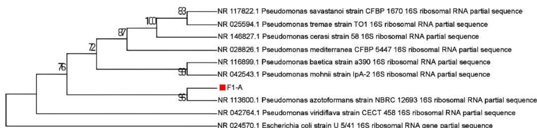
Figure 4. Construction of phylogeny tree of endophytic bacteria F1-A
