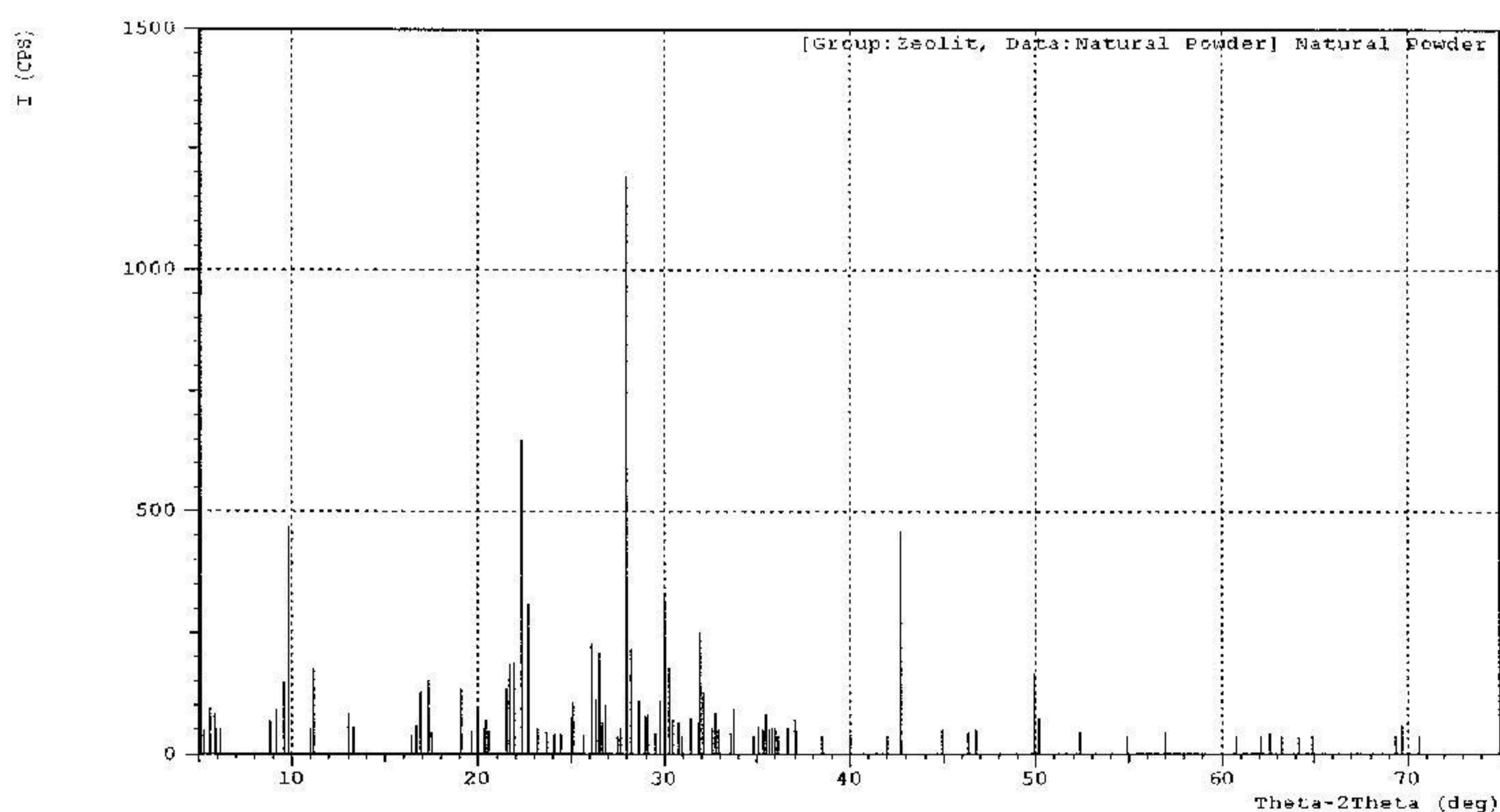
Fig.2. XRD Spectrum Line of Lampung Zeolit
