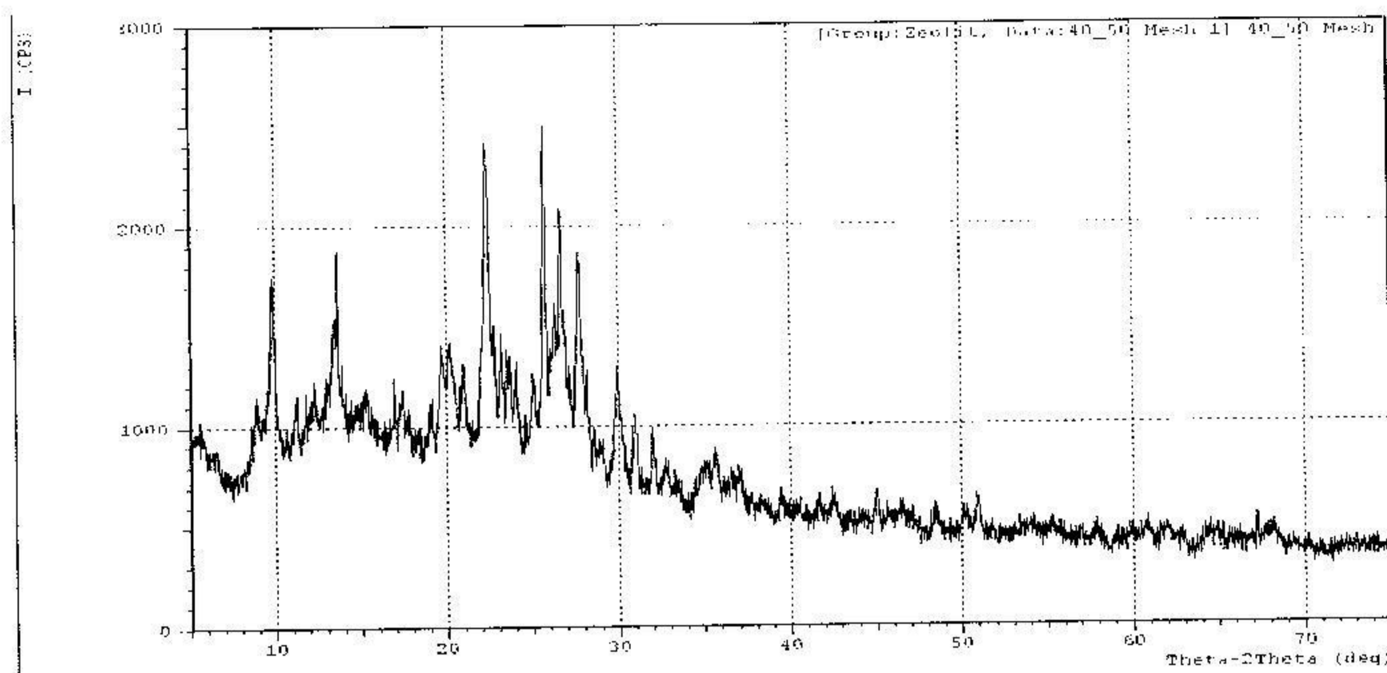
Fig.5. XRD Spectrum of Bayah, Banten Zeolit (40-50 mesh)
