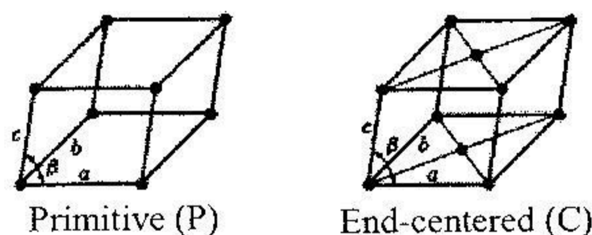
Fig.3. Bravais lattice for monoclinic crystal system.
