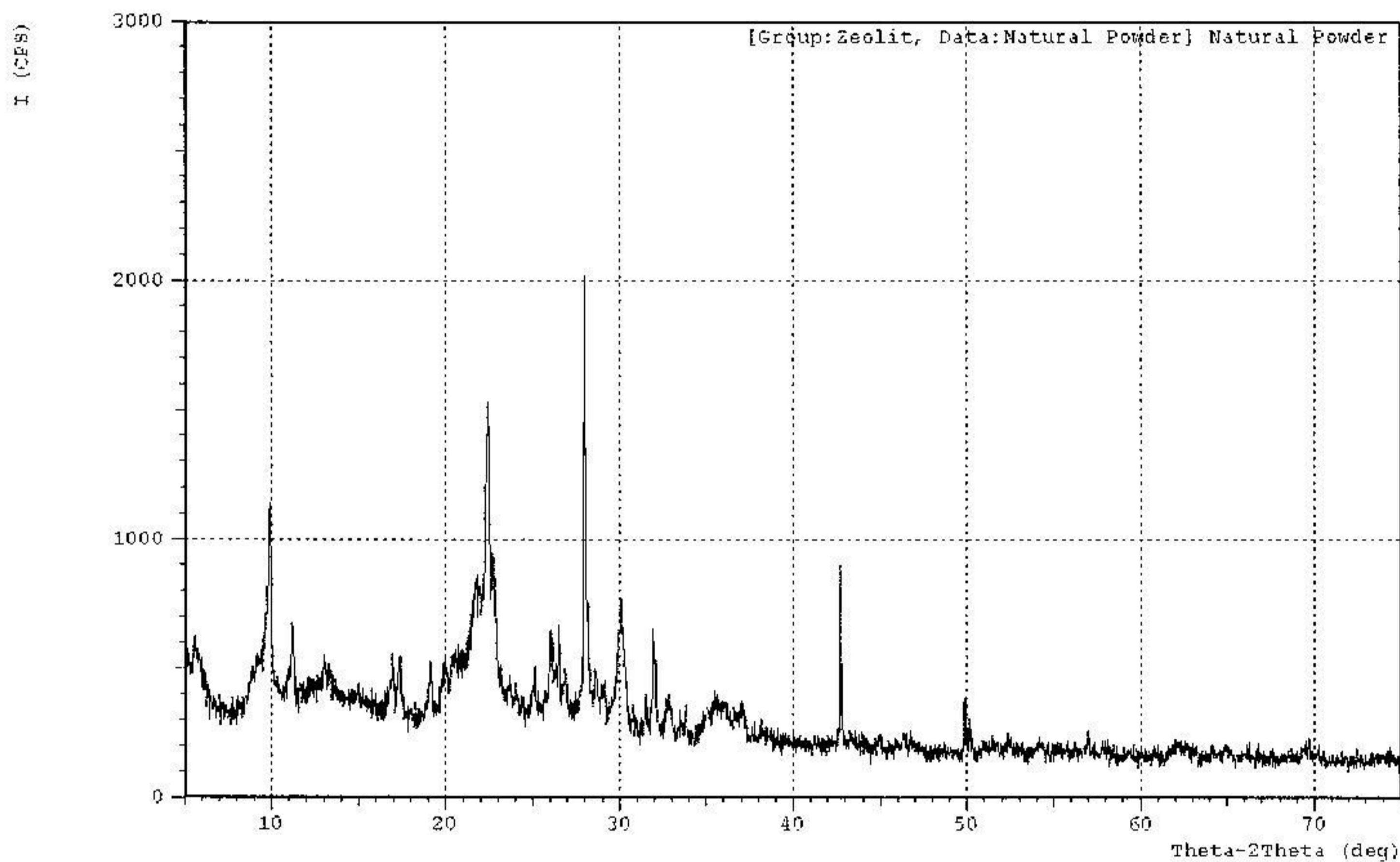
Fig.1. XRD Spectrum of Lampung Zeolit.
