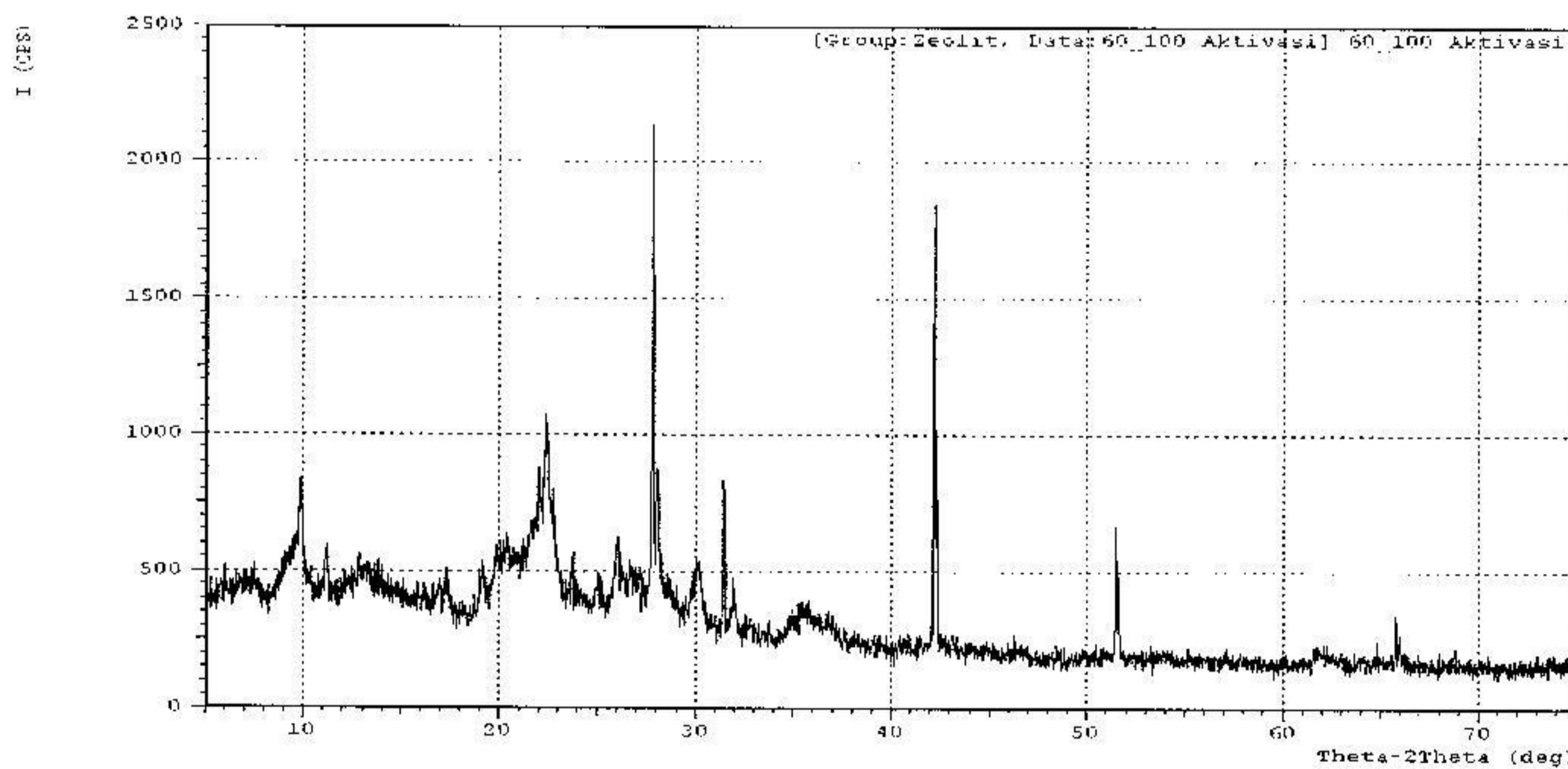
Fig.4. XRD spectrum of activated Lampung zeolit.
