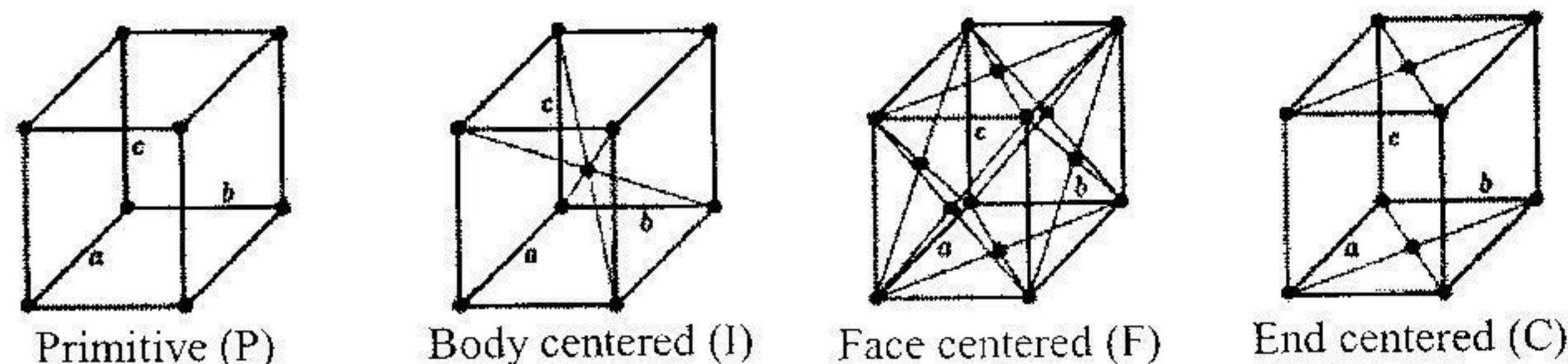
Fig.6. Bravais lattice of orthorhombic.
