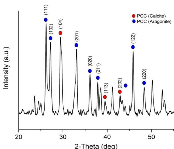
Figure 3. X-Ray diffraction pattern of the synthesized PCC
