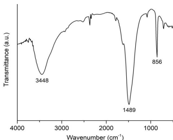
Figure 2. The IR spectra of the synthesized PCC
