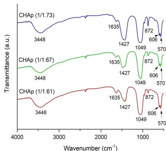
Figure 4. The IR spectra of the synthesized CHAp with 1.61, 1.67, and 1.73 Ca/P ratio
