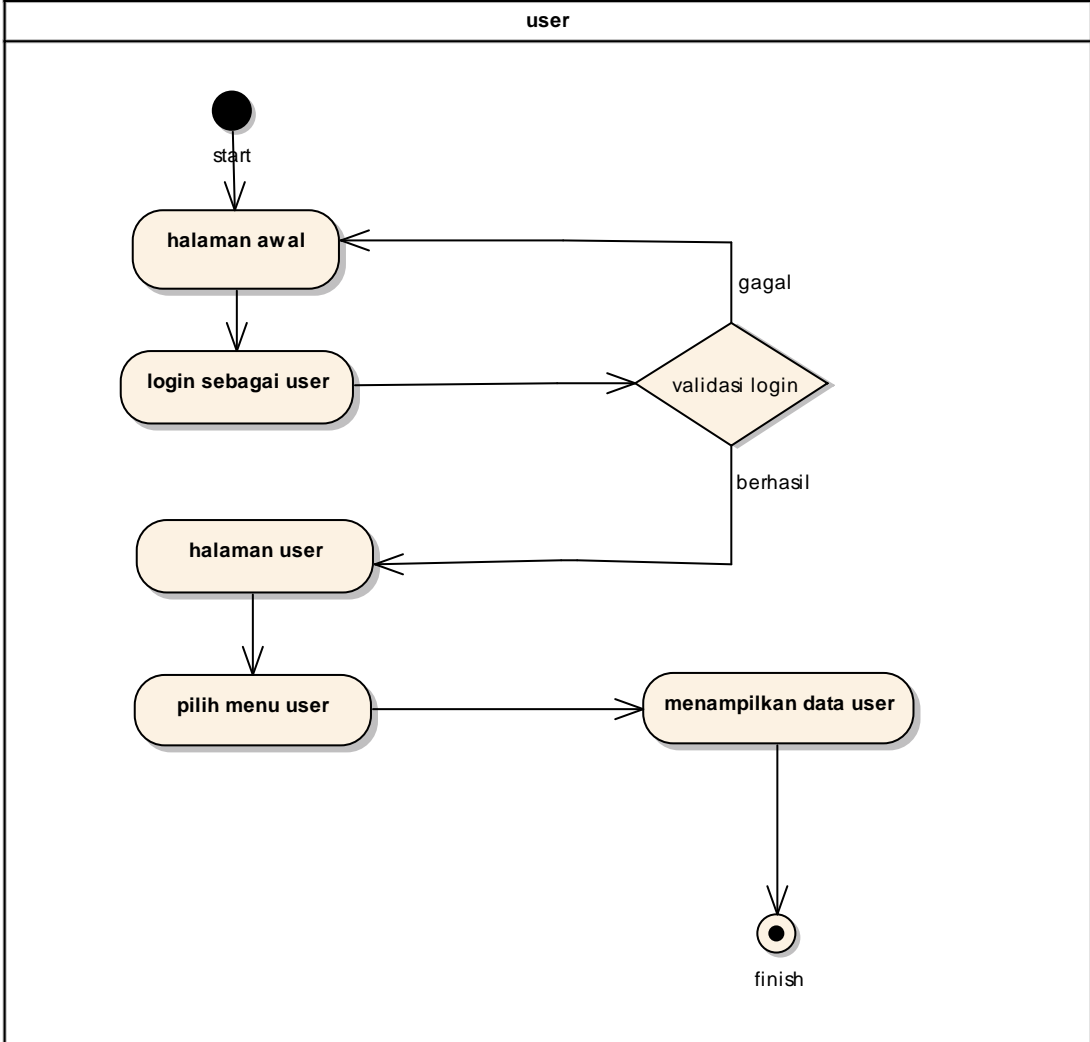
Gambar 4.4 Activity Diagram Login Use
