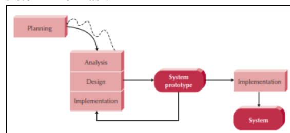
Gambar 5. Diagram Alir Metodologi Prototyping [9]
