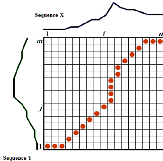
Gambar 3. Jarak Grid Global [4]
