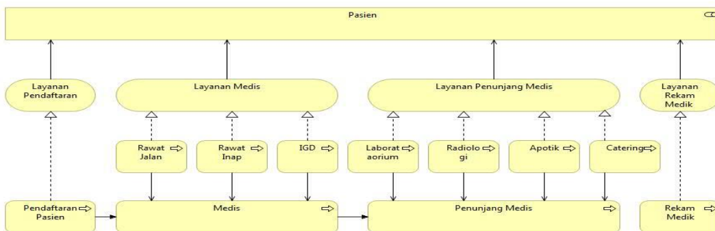
Gambar 4.3 Business Service
