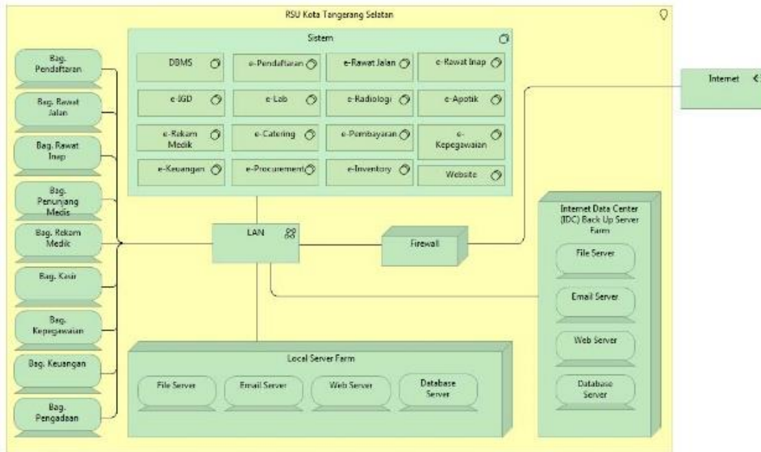
Gambar 4.6 Infrastructure Viewpoint
