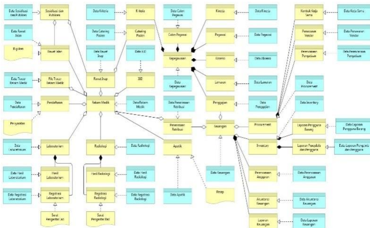
Gambar 4.4 Information Structure
