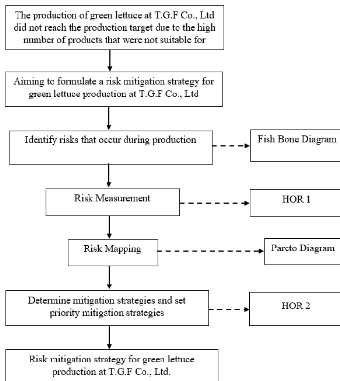
Figure 1. Framework Diagram
