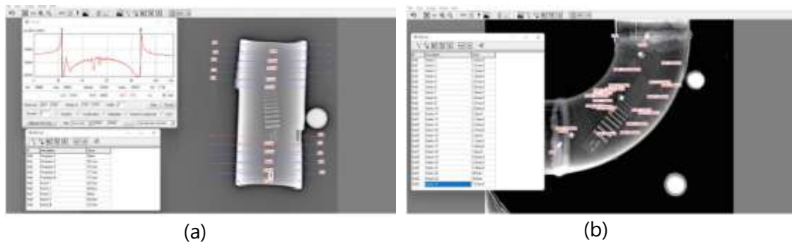
Figure 9. Dimension Defect Using Digital Detector Array on Pipes Artificial Defect (a), and Dimensions Defect on Insulated Pipe (b)
