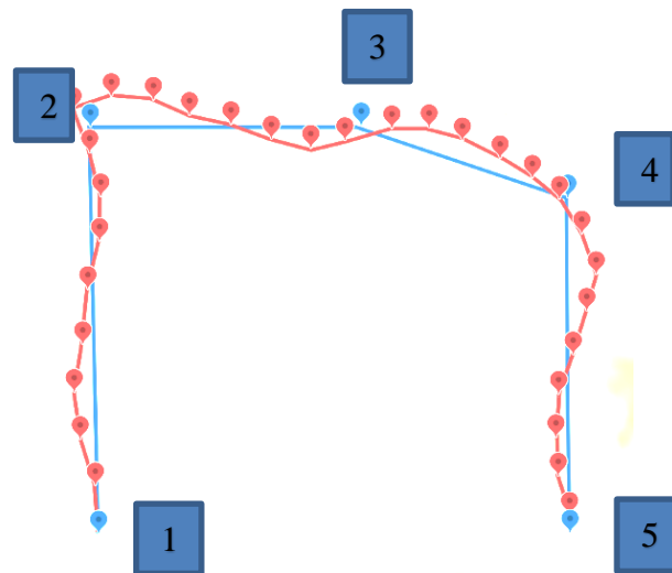
Figure 4. Tractor Prototype Path Plot Data
